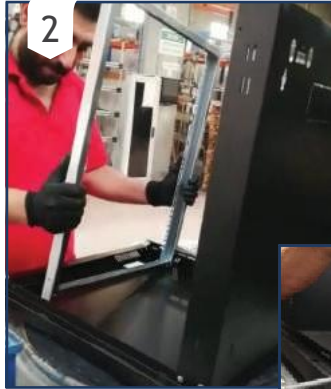
Base and Mounting Rails Assembly
